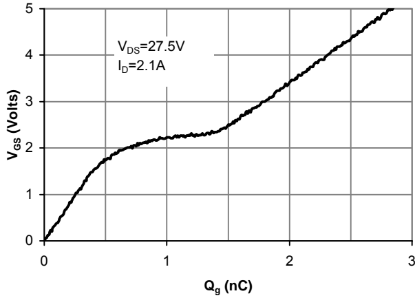
Figure 7: Gate-Charge Characteristics
