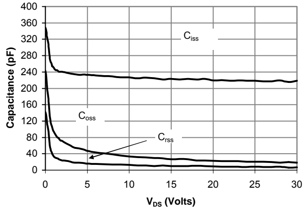
Figure 8: Capacitance Characteristics
